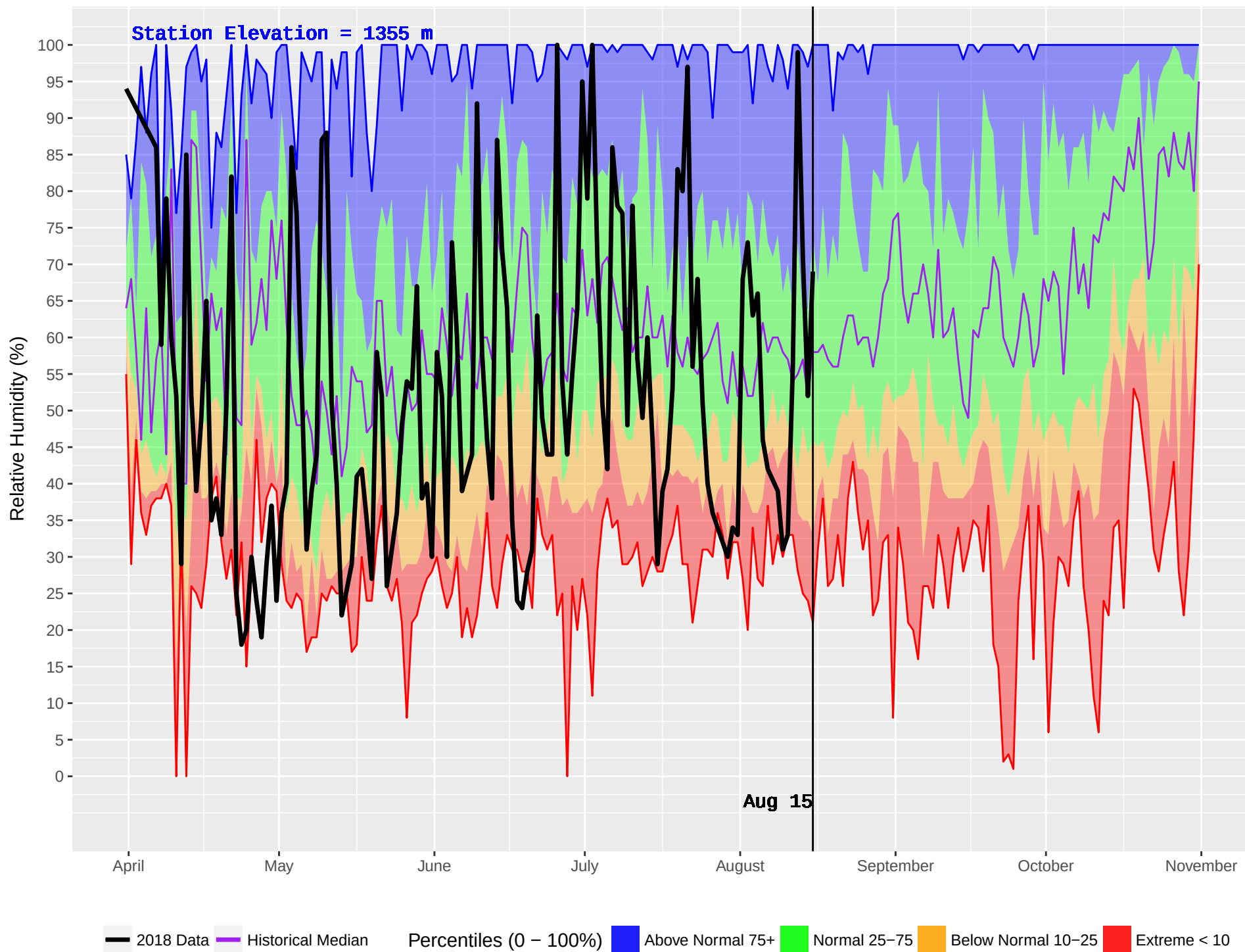
BIG VALLEY (262) : Historical (1987–2016) and Current (2018) Daily Relative Humidity
