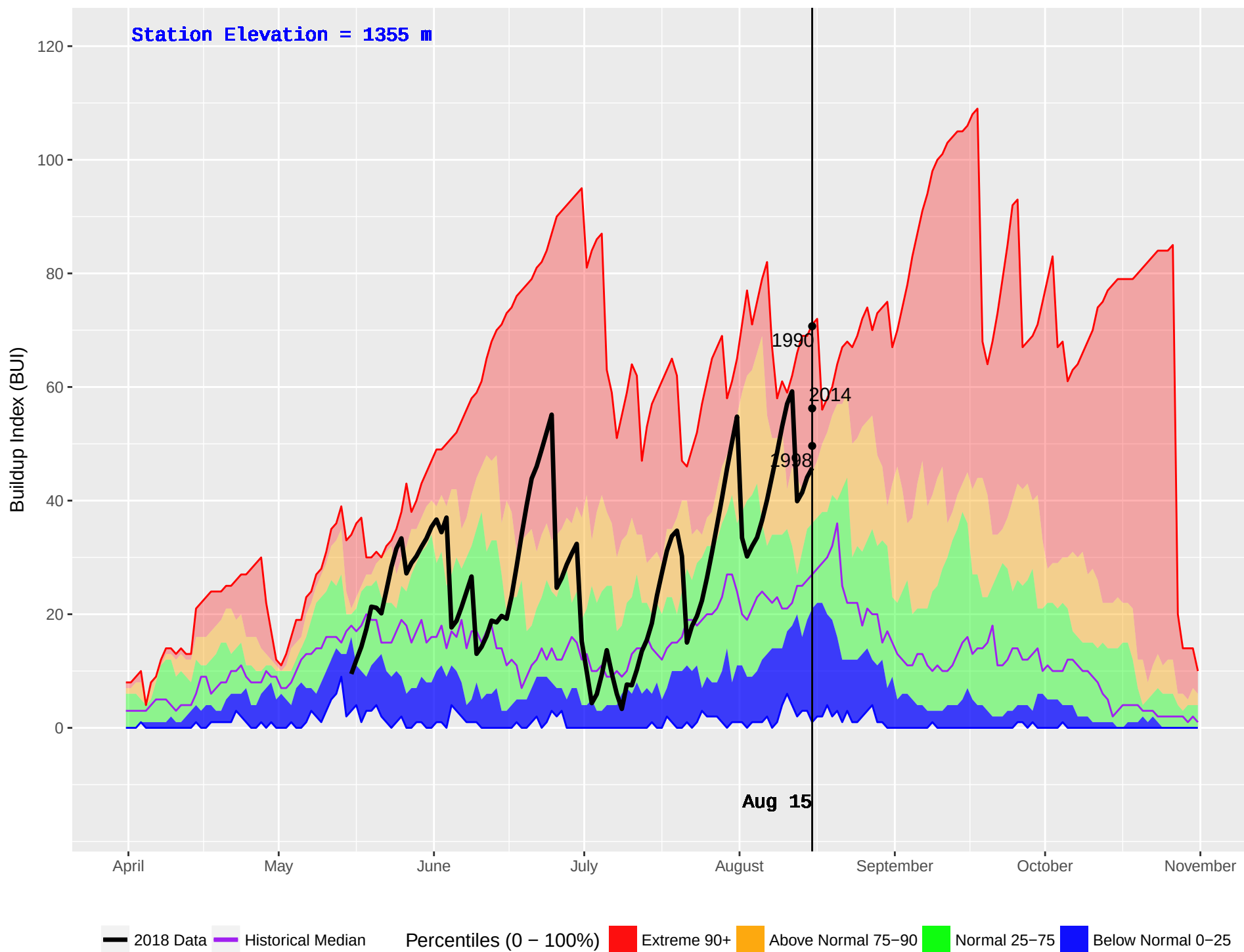
BIG VALLEY (262) : Historical (1987–2016) and Current (2018) Daily Buildup Index (BUI)
